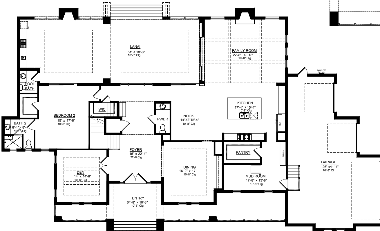
FIRST STORY
